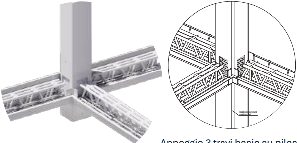
Appoggio 3 travi basic su pilastro pdti / Basic 3-beam support on PDTI pillar
