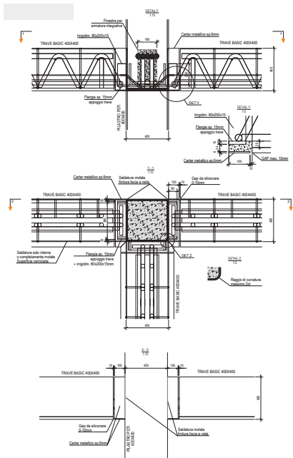
Appoggio 3 Travi Basic su Pilastro Pdti / Basic 3-Beam Support on PDTI Pillar
