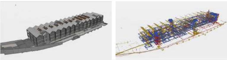
Modello BIM - Strutture / BIM model - Structures
