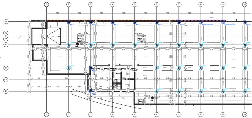
Pilastri - Pianta Pilastri L-1 e L00, fili 1-10 / Pillars - Plan Pillars L-1 and L00, wires 1-10
