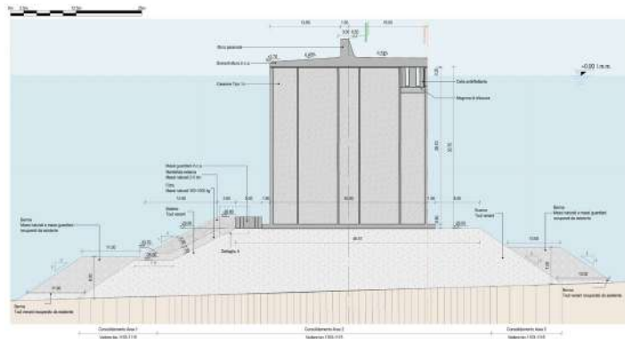
Cassoni layout / Layout containers
