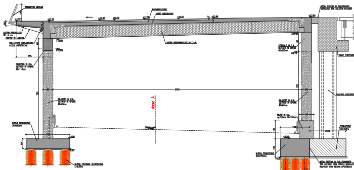
Sezione galleria e varo travi galleria / Tunnel section and installation of tunnel beams
